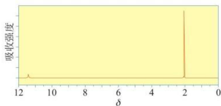
图3-23 乙酸的核磁共振氢谱
