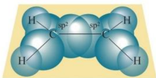
\sigma 键
