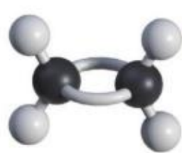
乙烯
