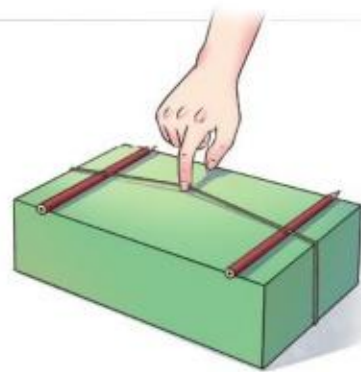
图2.1-2 拨动橡皮筋
